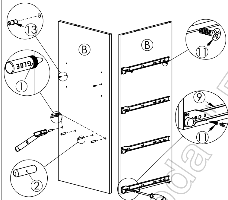
Korak 3
