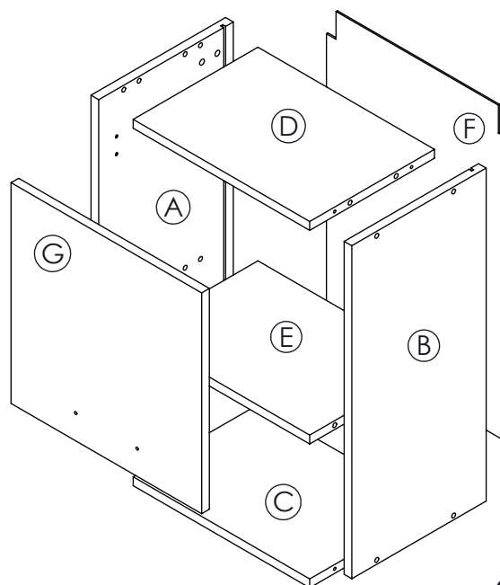
Korak 3
