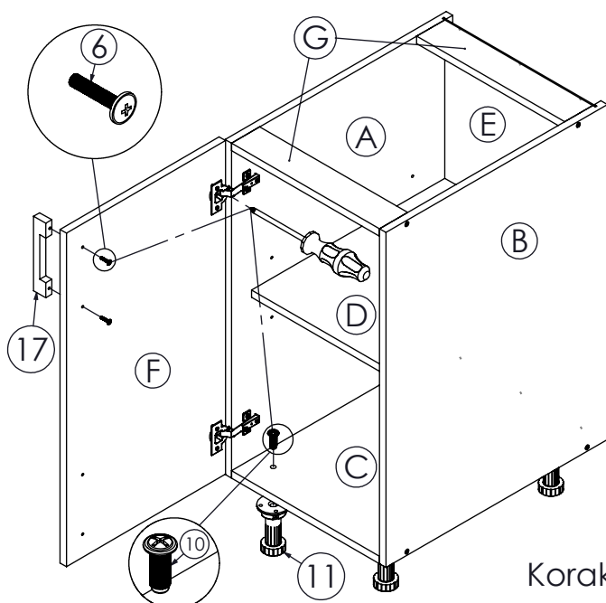
Korak 3
