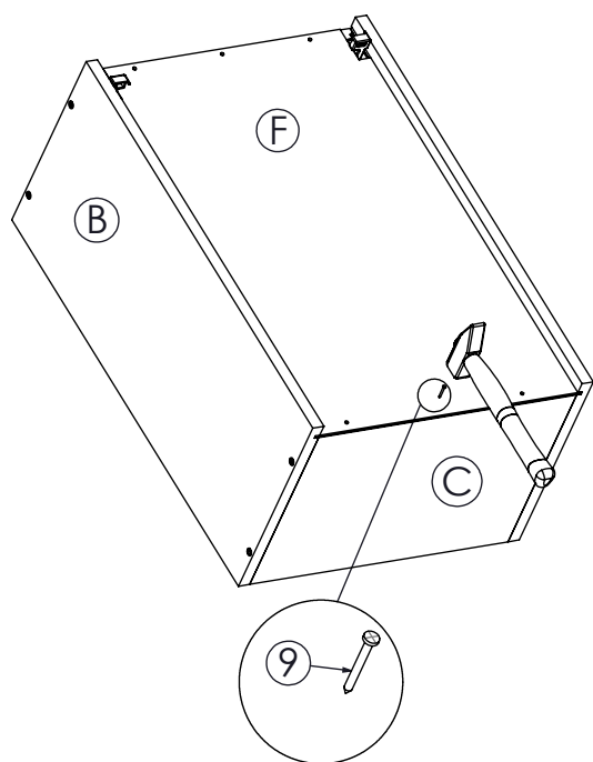
Korak 3
